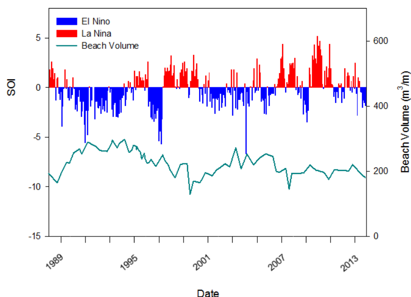
Figure 4-13 Displaying ENSO trends measured by SOI values since 1987, with El Nino represented by blue bars and La Nina in red at the top, and averaged beach-wide volume oscillations at Pakiri are in teal on the bottom. Note the two main cyclic phases of El Nino (between 1989 and 1996; and 2000 and 2006) correspond to increases in beach volume (Source: http://www.cpc.ncep.noaa.gov/data/indices/soi ).
