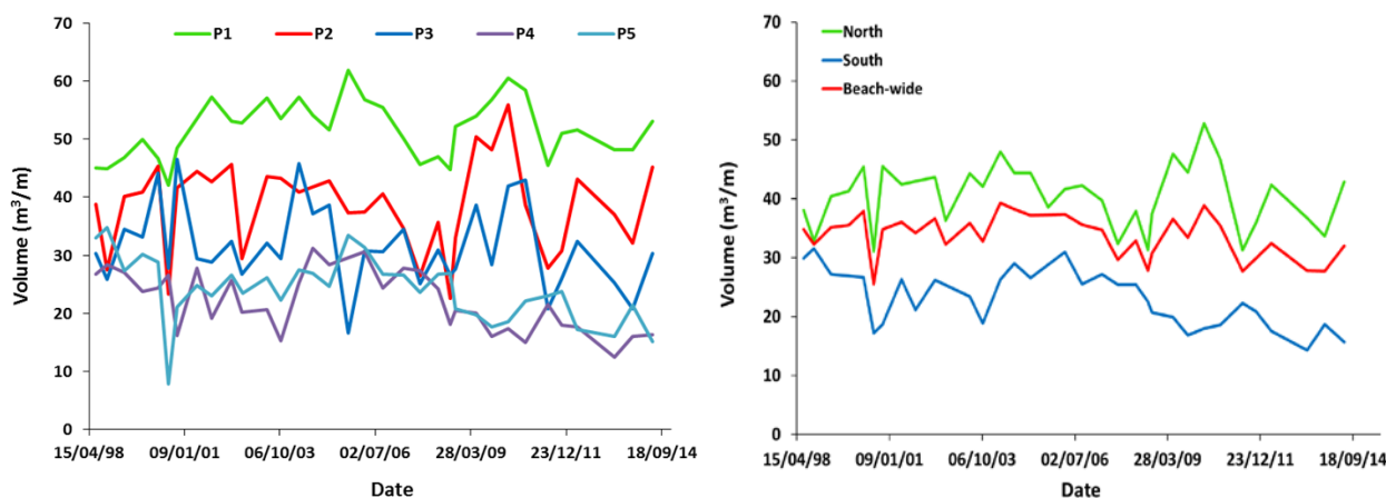
Figure 8-8 Beach volume changes at the MSL contour at Milford Beach, showing individual profile time series on the left, and the combined beach-wide, northern and southern averaged volumes time series on the right.
