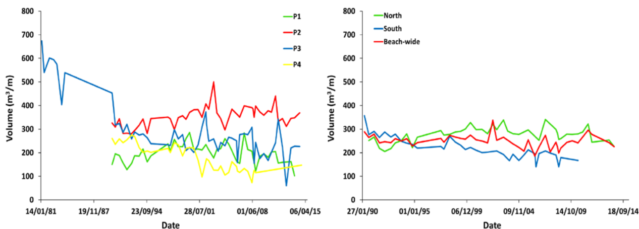
Figure 4-5 Beach volume changes at the 1m contour at Muriwai, showing individual profile time series on the left, and the combined beach-wide, northern and southern averaged volume time series on the right.
