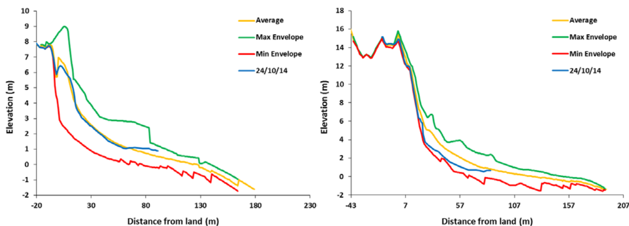
Figure 4-7 Beach profile envelope of Profiles 2A (left) and 6 (right), illustrating the average beach profile in orange, the maximum extent of all profiles in green, the minimum extent of all profiles in red and, the most recent beach profile in blue. These profiles are indicative of the other profile envelopes in the northern and southern sections of the beach.
