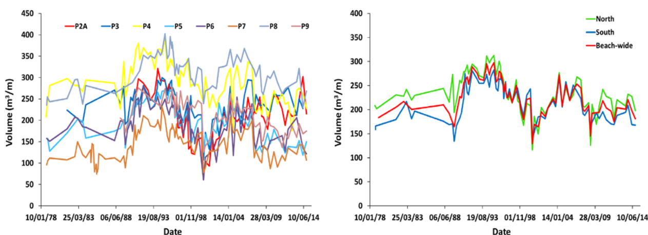
Figure 4-8 Beach volume changes at the 1m contour at Pakiri, showing individual profile time series on the left, and combined beach-wide, northern and southern averaged volume time series on the right.
