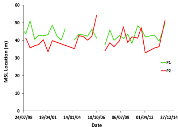
Figure 8-6 Beach width changes at the MSL contour. Profile 1 is in green and profile 2 is in red.
